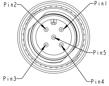
C1 Pin Assignments Front View
