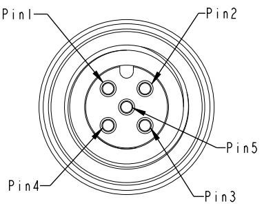
C2 Pin Assignments Front View
