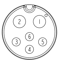
C2 Pin Assignments Front View
