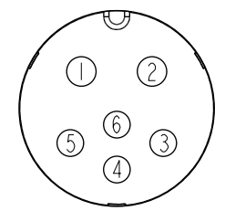
C1 & C2 Pin Assignments Front View
