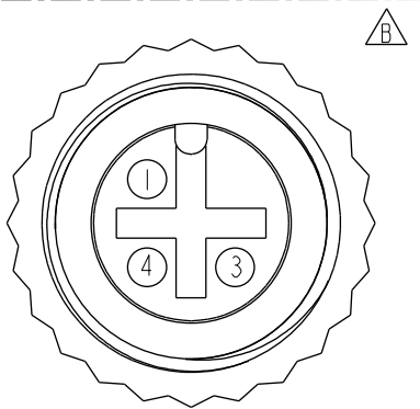
Conn. 1 & 2 Pin Assignments Front View
